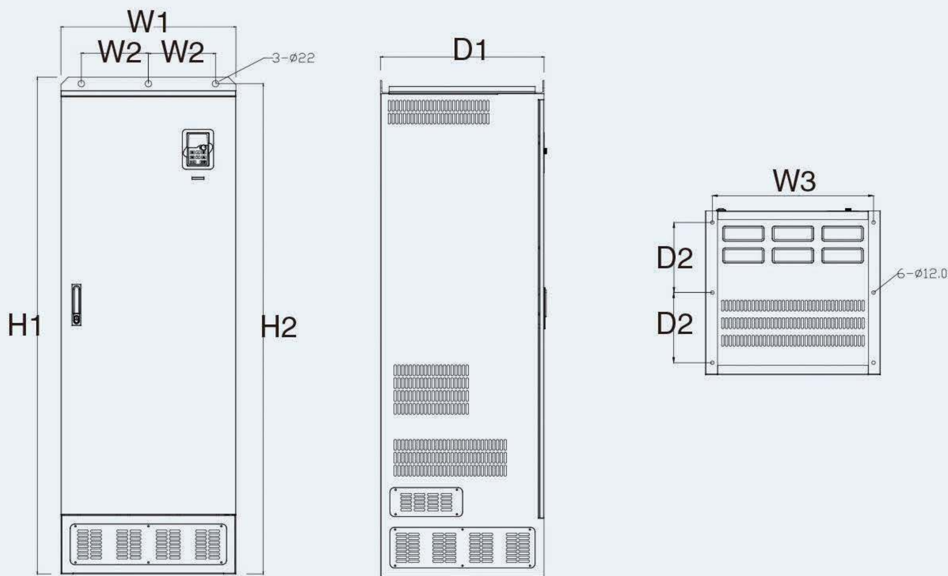
Floor mounting for the 355-500kW models
