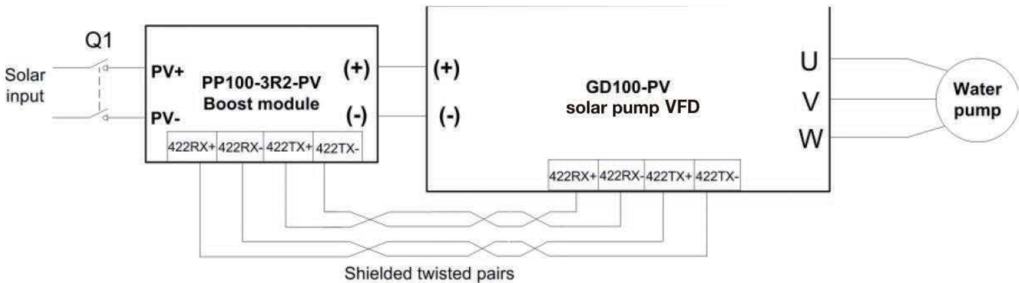
Connection between the boost module and solar pumping VFD
