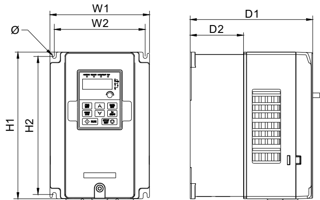
Wall mounting
