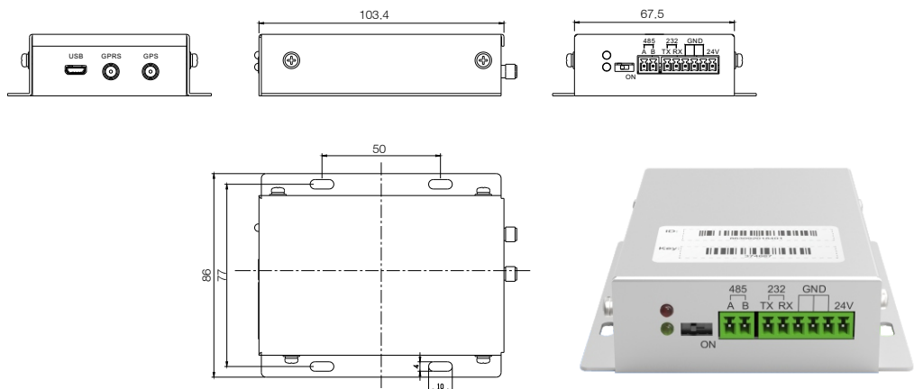
GPRS module installation dimensions
