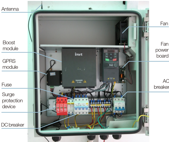
Internal structure of GD100-2R2G-S25-PV-AS
