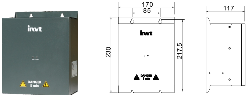
Installation dimension
