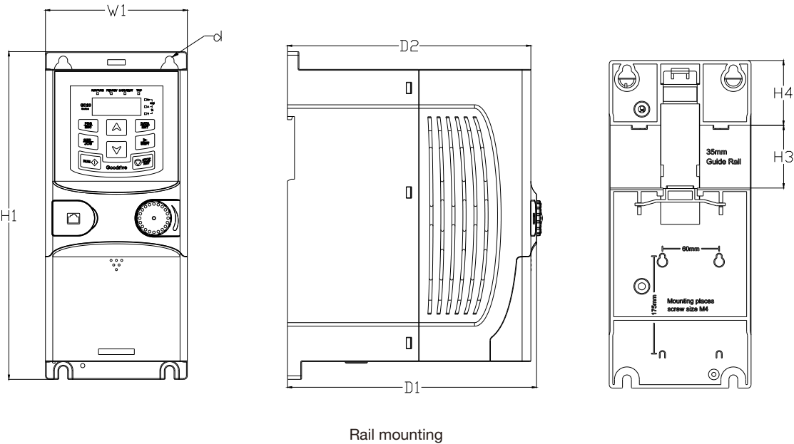
Rail mounting
