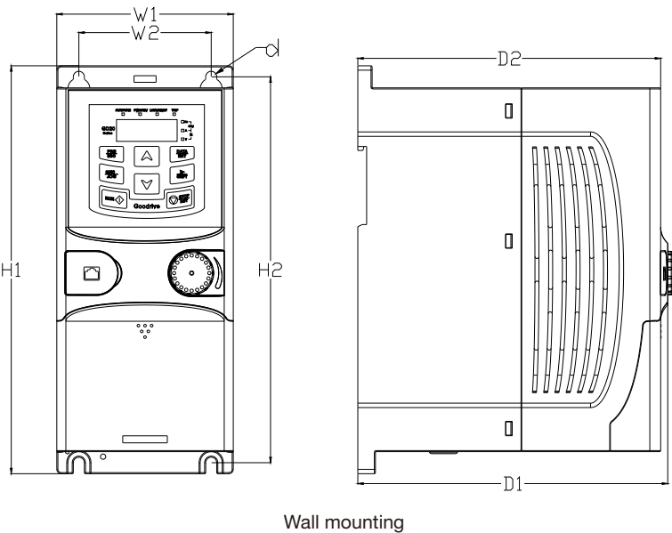
Wall mounting
