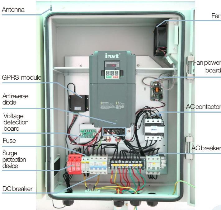
Internal structure of GD100-015G-45-PV-AS
