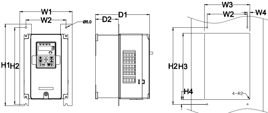
Flange installation
